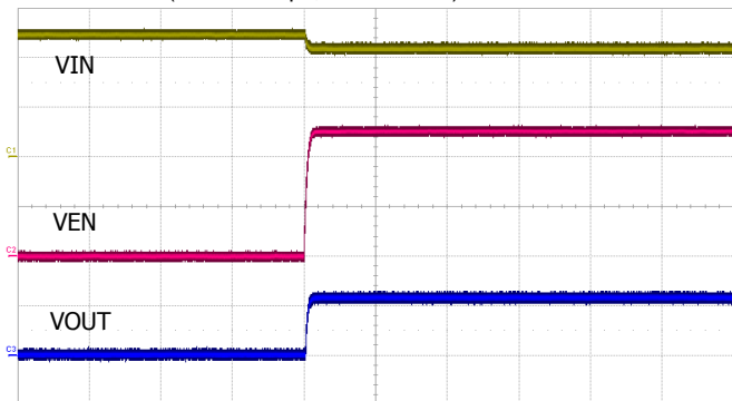
VIN : 1.0V/div, VEN : 1.0V/div, VOUT : 1.0V/div, Time : 5ms/div Start Up by External VEN @ Iout=2A
